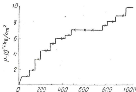
FIG. 3. Graph of cerium specimen held in apparatus under pressure (in one series of experiments); × - exposure time.
